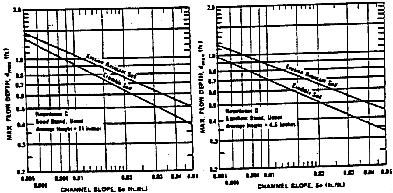
MAXIMUM PERMISSIBLE DEPTH OF FLOW ( d_{max} ) FOR CHANNELS LINED WITH COMMON LESPEDEZA OF VARIOUS LENGTHS
