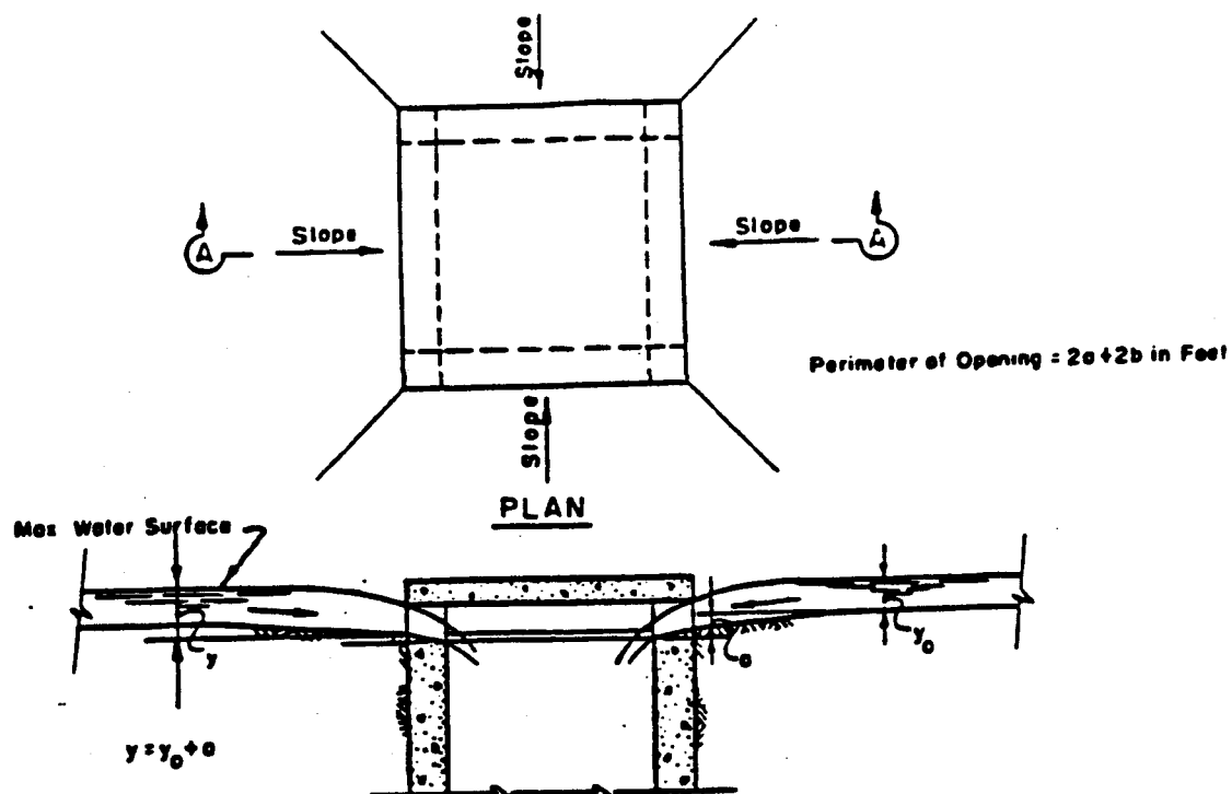
SECTION A-A DROP INLET TYPE A-4
