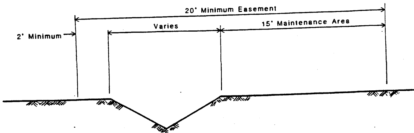
SMALL DITCH
