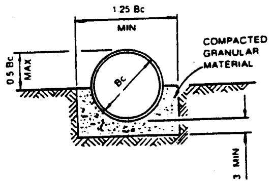
GRANULAR FOUNDATION
