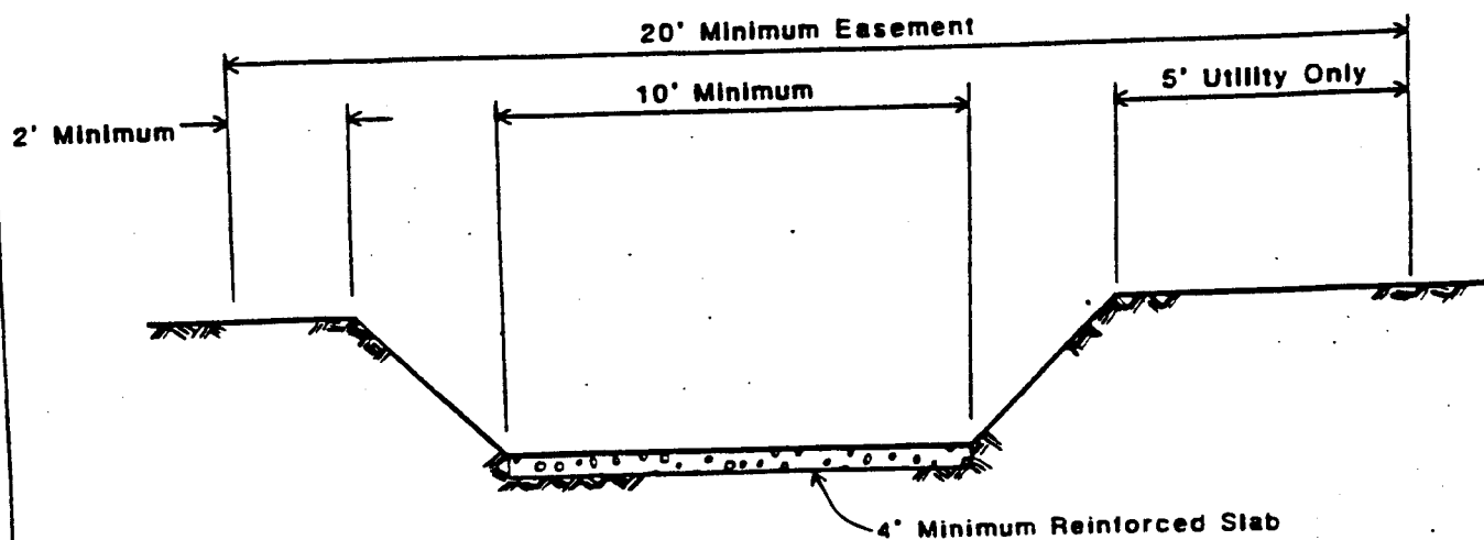
LARGE DITCH
