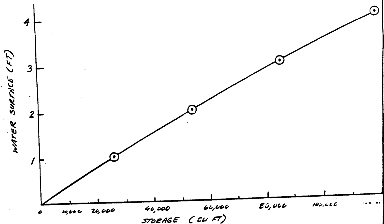
STAGE-STORAGE GRAPH (FROM TABLE 1)
