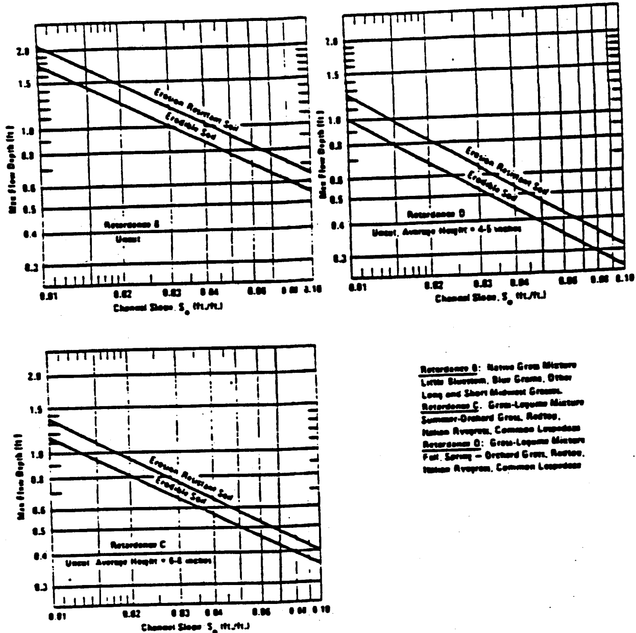
Maximum Permissible Depth of Flow ( d_{max} ) for Channels Lined with Grass Mixtures. Good Stand, Uncut
