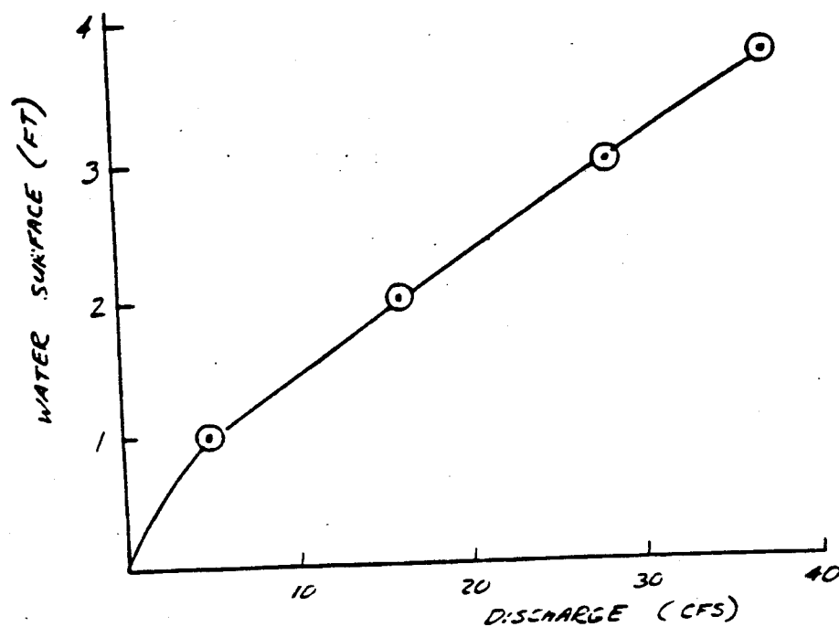
STAGE-DISCHARGE GRAPH (FROM TABLE 2)
