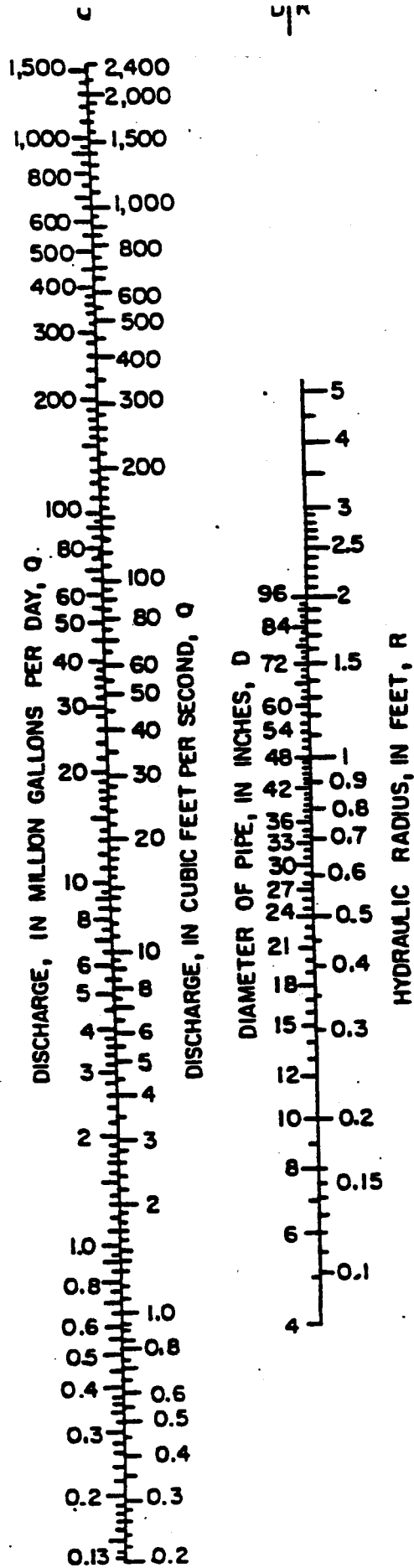
Nomograph for solution of the Manning formula.
