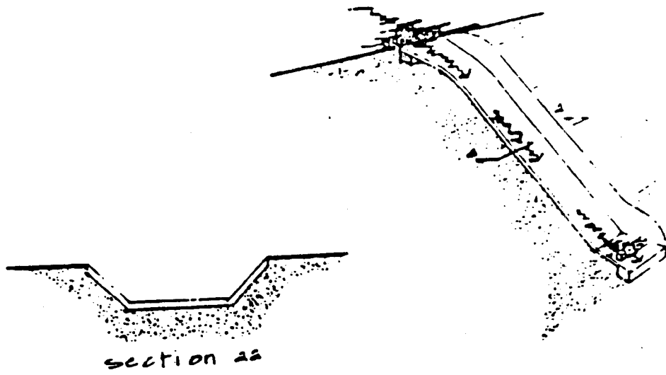
Down drain
