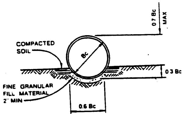
SHAPED SUBGRADE AT GRANULAR FOUNDATION
