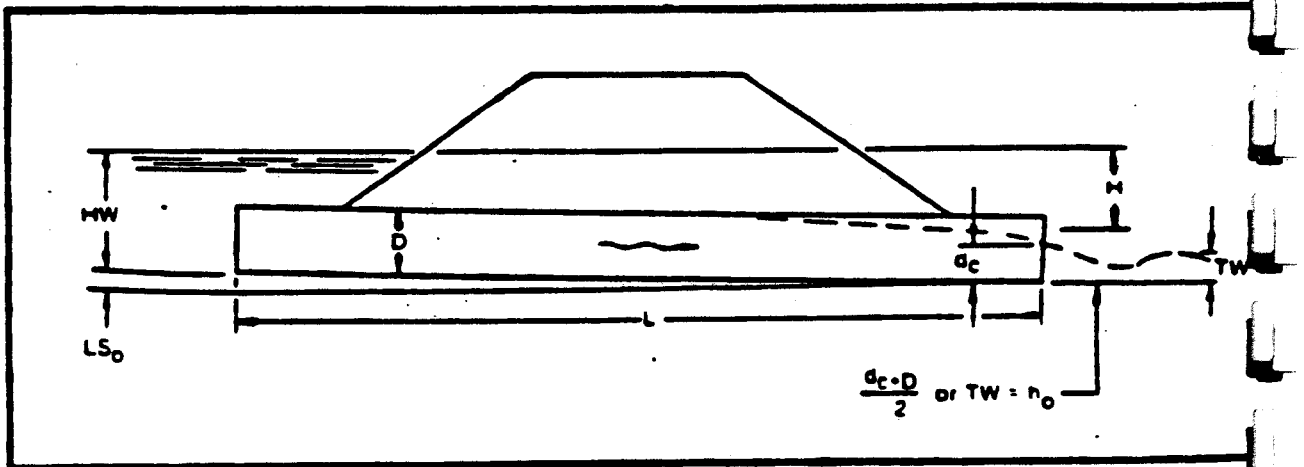
OUTLET CONTROL
