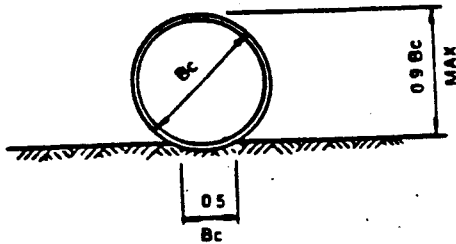
SHAPED SUBGRADE
