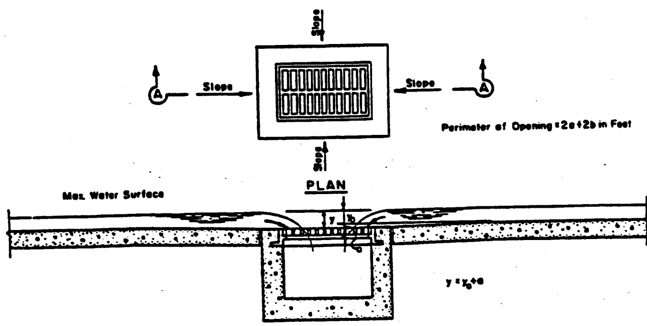
SECTION A-A DROP INLET (Grate covering) TYPE A-5
